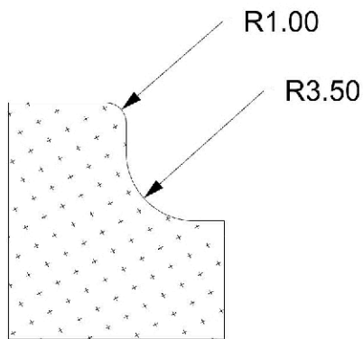
Curb Profile
