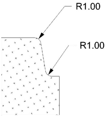
Curb Profile
