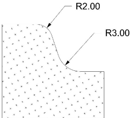
Curb Profile
