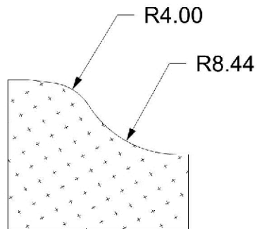
Curb Profile
