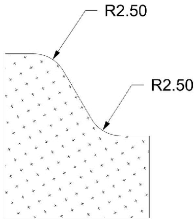
Curb Profile
